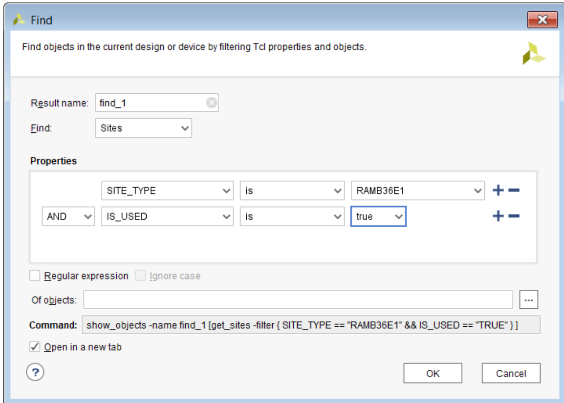
Figure 15: Finding Placed RAMB36 Cells
