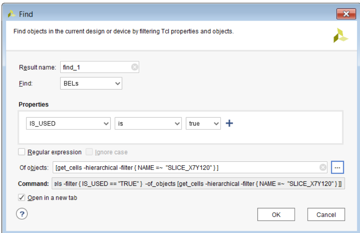
Figure 17: Finding Occupied BELs within a Slice
