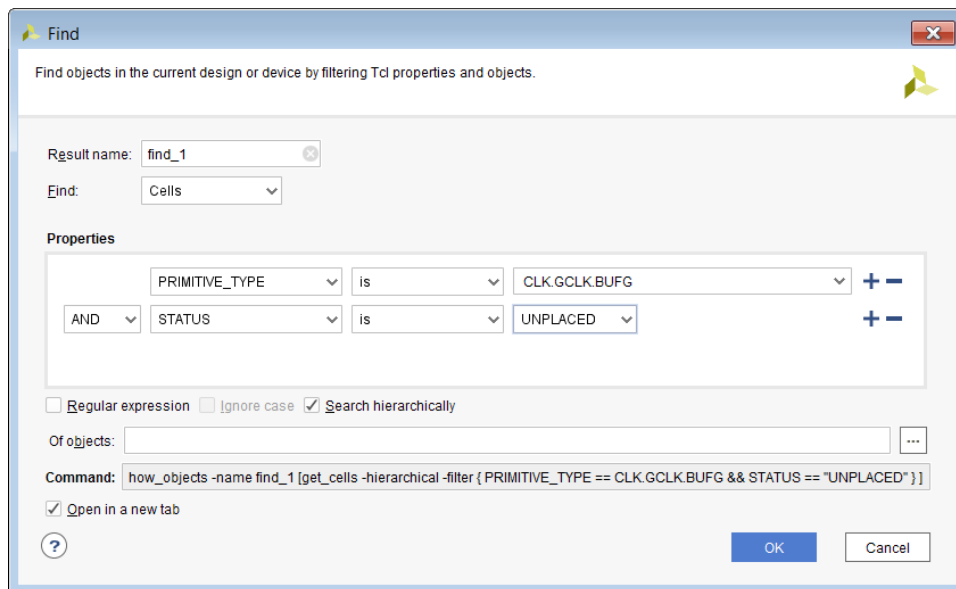
Figure 13: Finding Unplaced BUFGs
