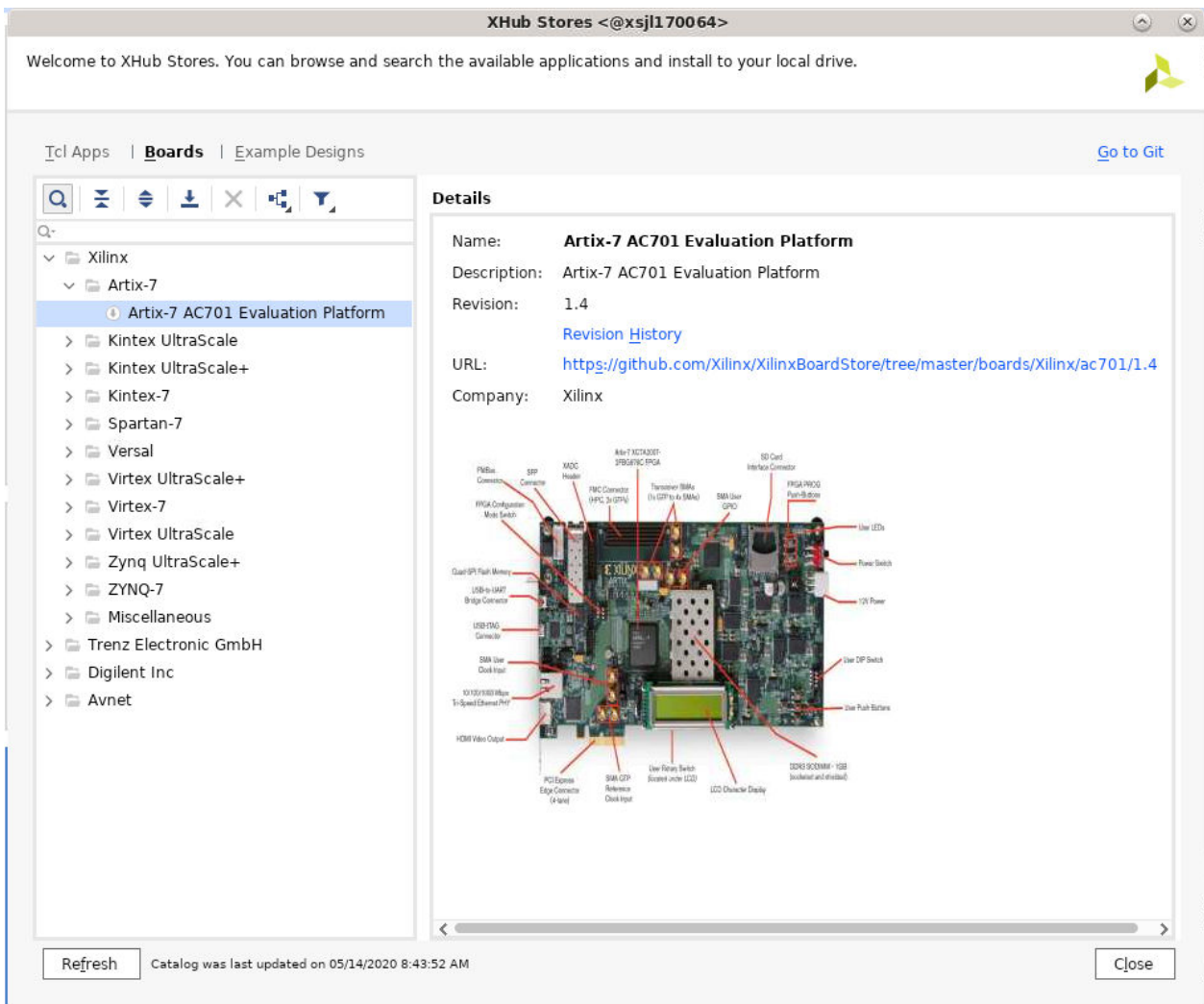
Figure 3: XHUB Stores
