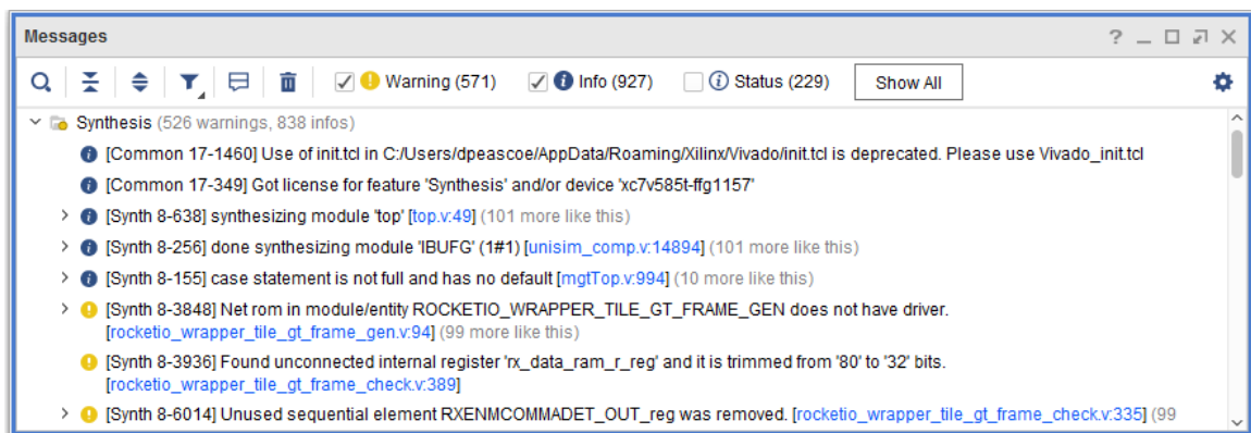
Figure 67: Messages Window
