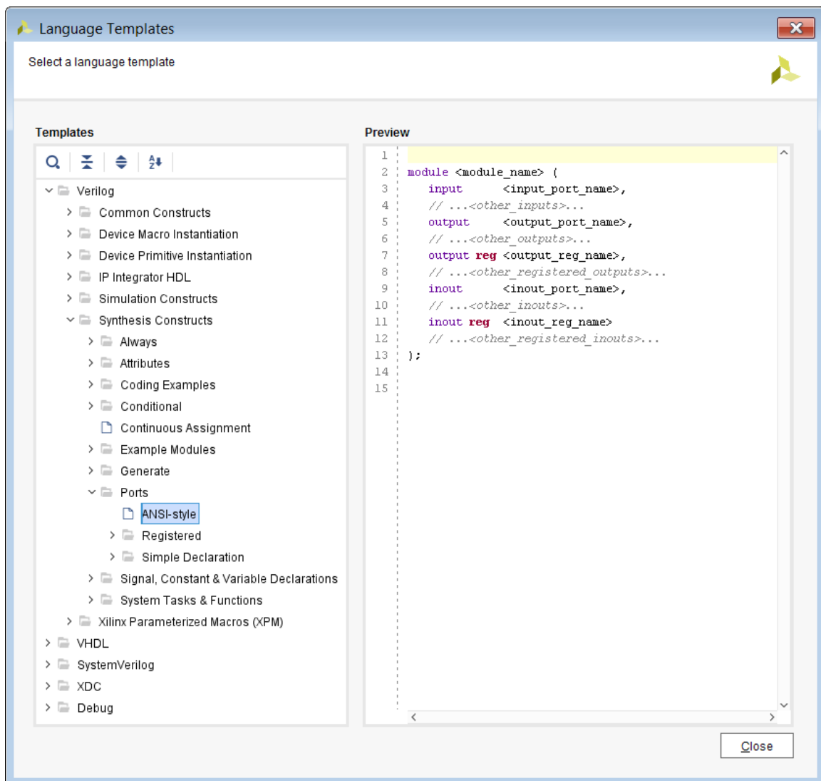
Figure 9: Language Templates
